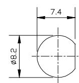
PUNCH DETAIL
